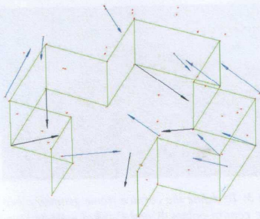
Figure 4: Residual vectors of the alignment points magnified with a scale factor of 100.
