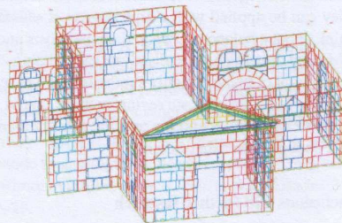
Figure 2: Partial 3d CAD model resulting from drawing rectification.
