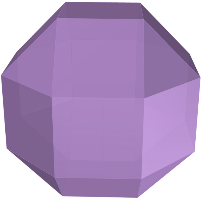
Rombicuboctaedro
