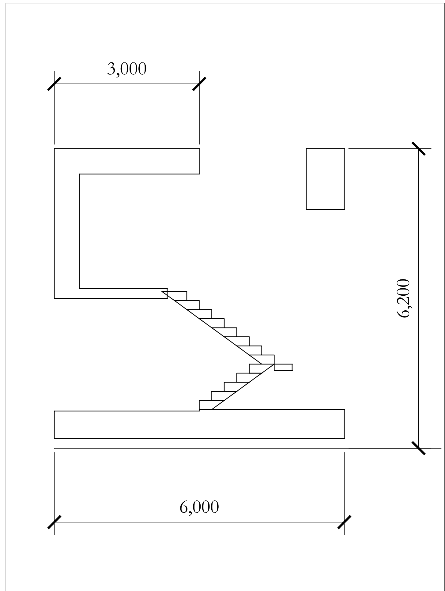
Corte Vertical 1:100
