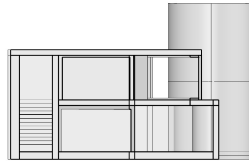
CORTE VERTICAL
