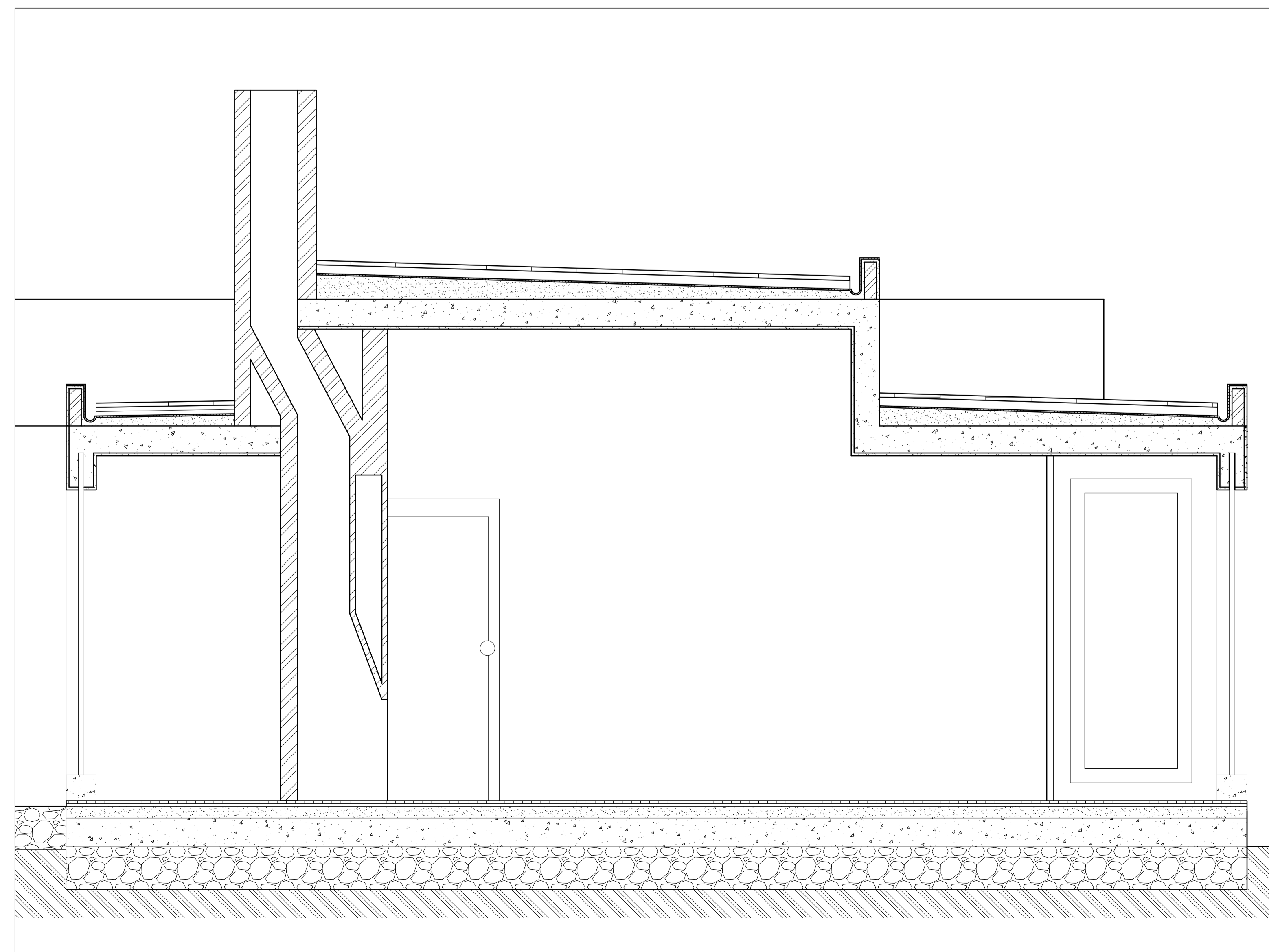
PORMENOR AA' 1:20
