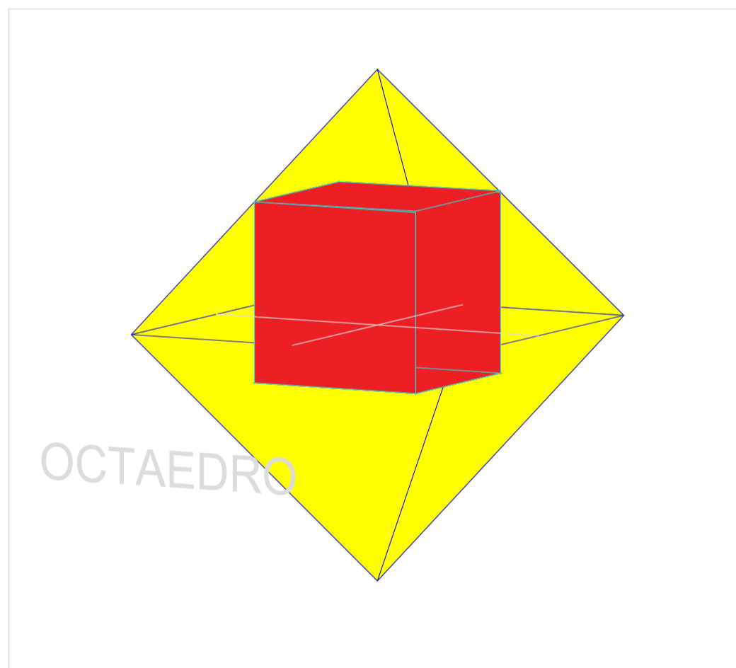
Octaedro
