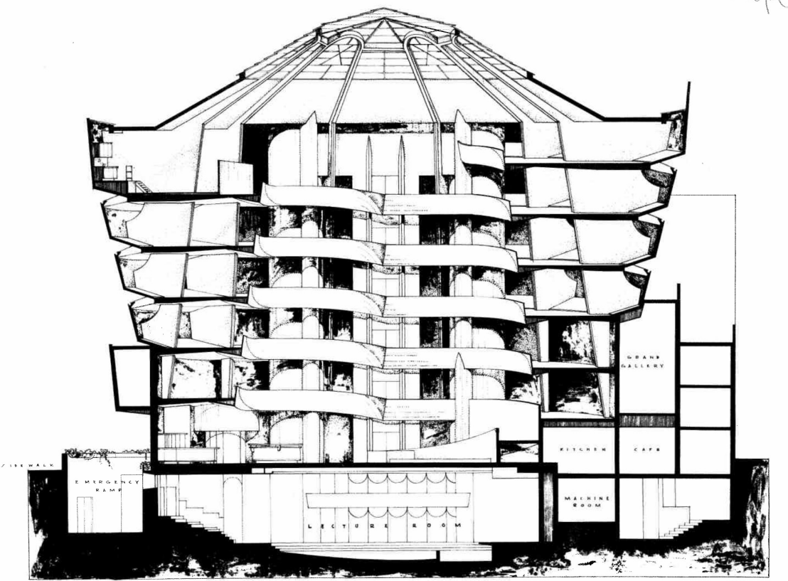
SECTION THROUGH MAIN GALLERY THE SOLOMON R. GUGGENHEIM MUSEUM FRANK LLOYD WRIGHT ARCHITECT
