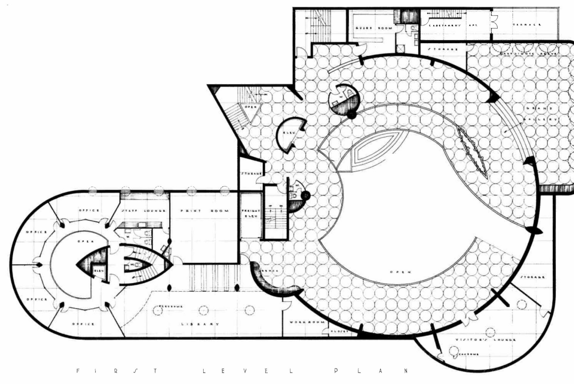
FIRST LEVEL PLAN THE SOLOMON R. GUGGENHEIM MUSEUM FRANK LLOYD WRIGHT ARCHITECT
