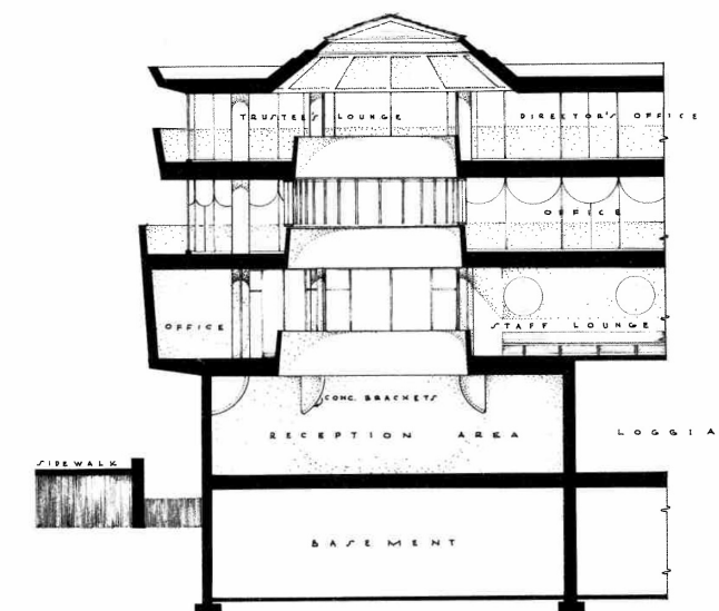
SECTION THROUGH ADMINISTRATION BUILDING THE SOLOMON R. GUGGENHEIM MUSEUM FRANK LLOYD WRIGHT ARCHITECT
