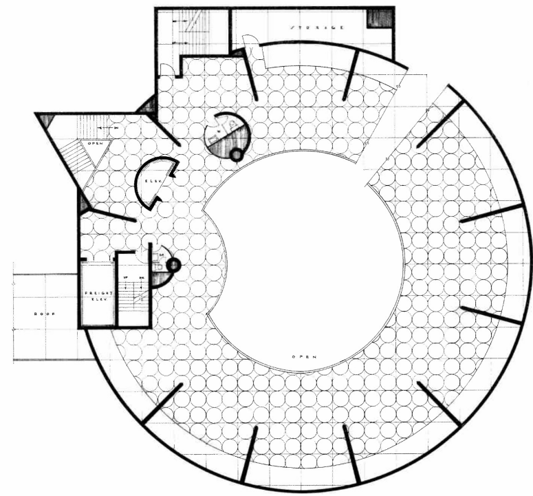
FOURTH LEVEL PLAN THE SOLOMON R. GUGGENHEIM MUSEUM FRANK LLOYD WRIGHT ARCHITECT
