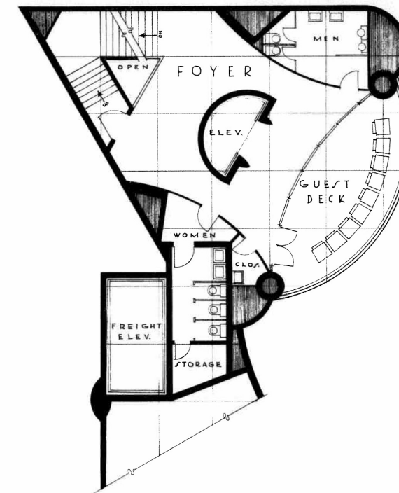
PLAN OF MEZZANINE THE SOLOMON R. GUGGENHEIM FOUND MUSEUM FRANK LLOYD WRIGHT ARCHITECT
