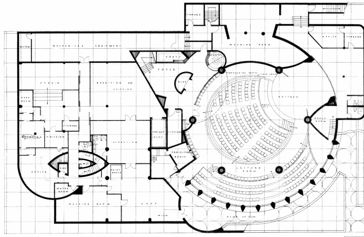
BASEMENT PLAN THE SOLOMON R. GUGGENHEIM MUSEUM FRANK LLOYD WRIGHT ARCHITECT
