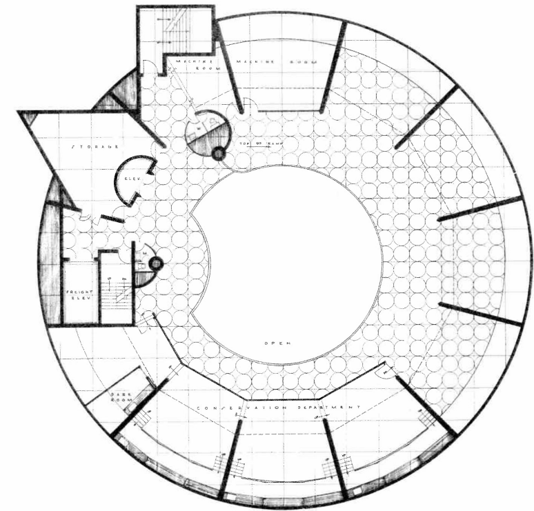
FIFTH LEVEL PLAN THE SOLOMON R. GUGGENHEIM MUSEUM FRANK LLOYD WRIGHT ARCHITECT
