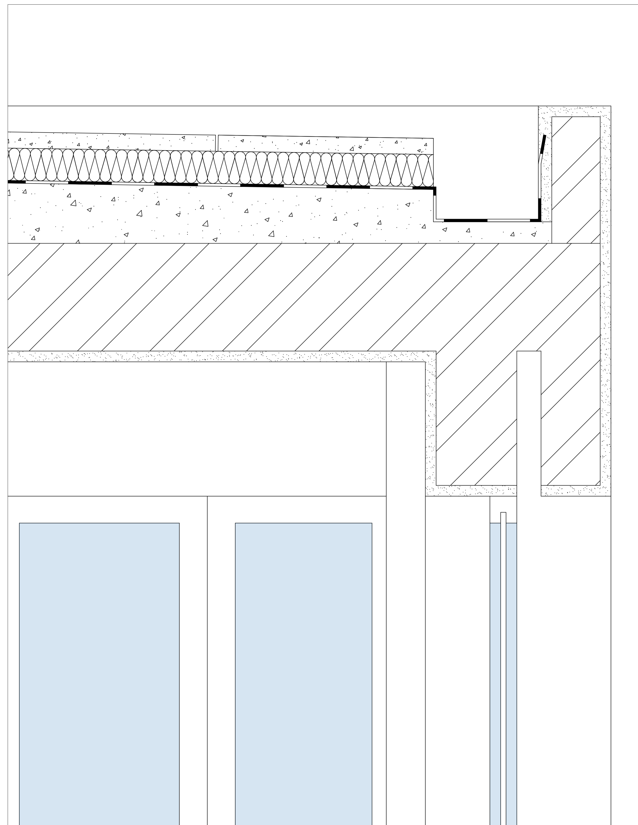
Ceiling Details 1:5
