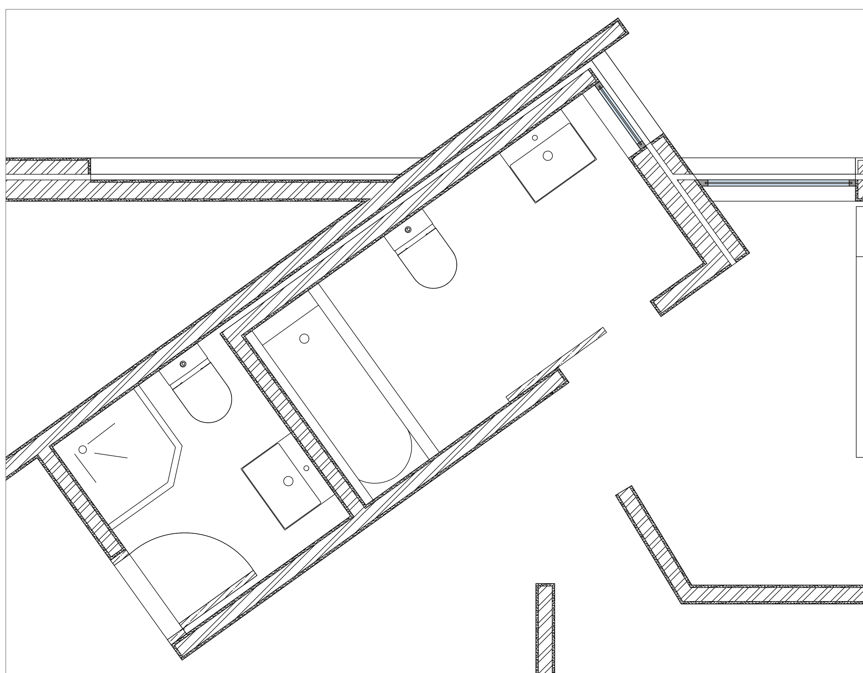
S.I Equipments 1:20
