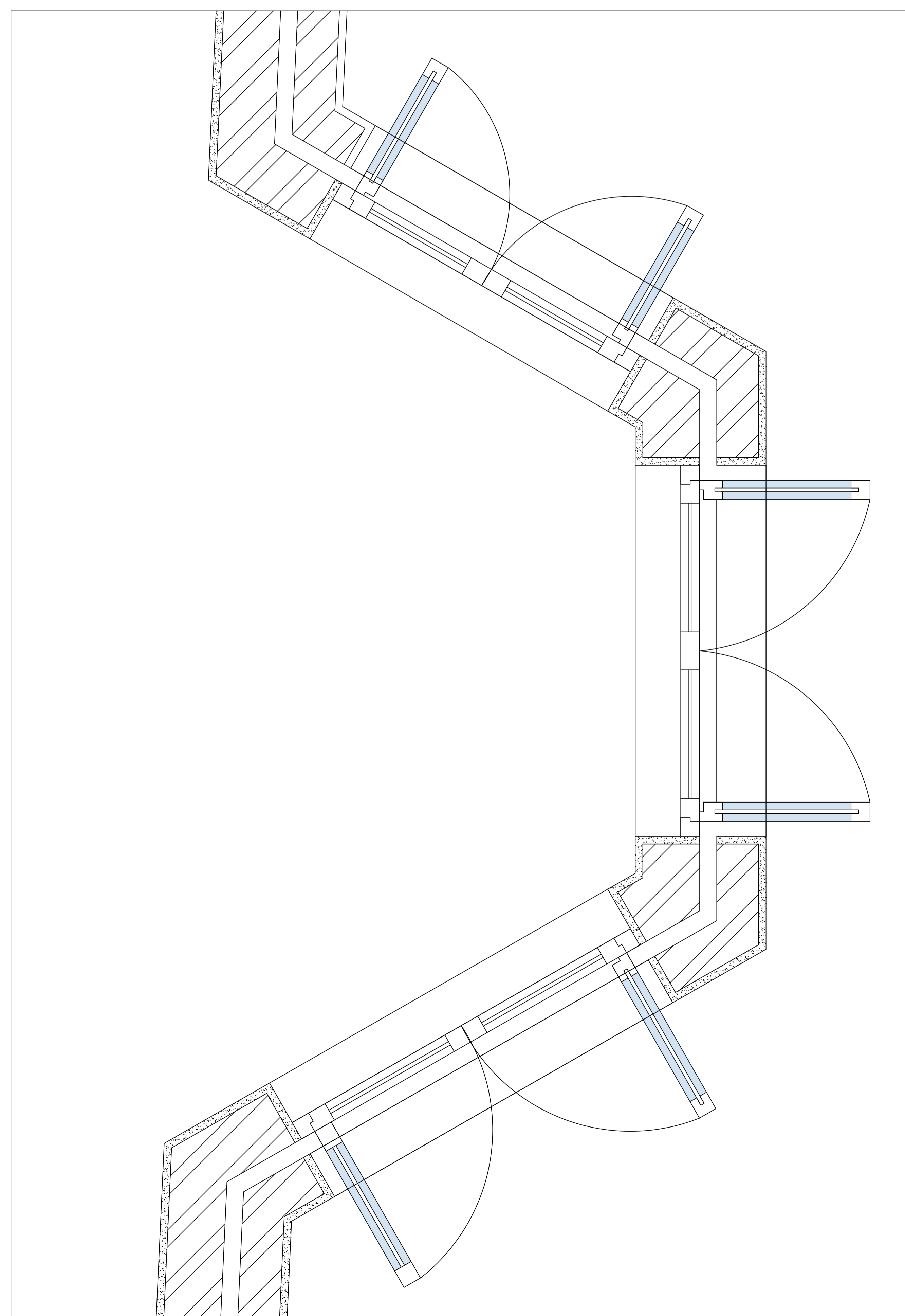
Windows Details 1:10
