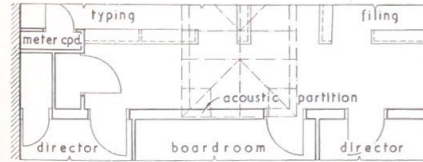
LAYOUT PLAN SHOWING ACOUSTIC PARTITION. scale 1/8" = 1'-0"
