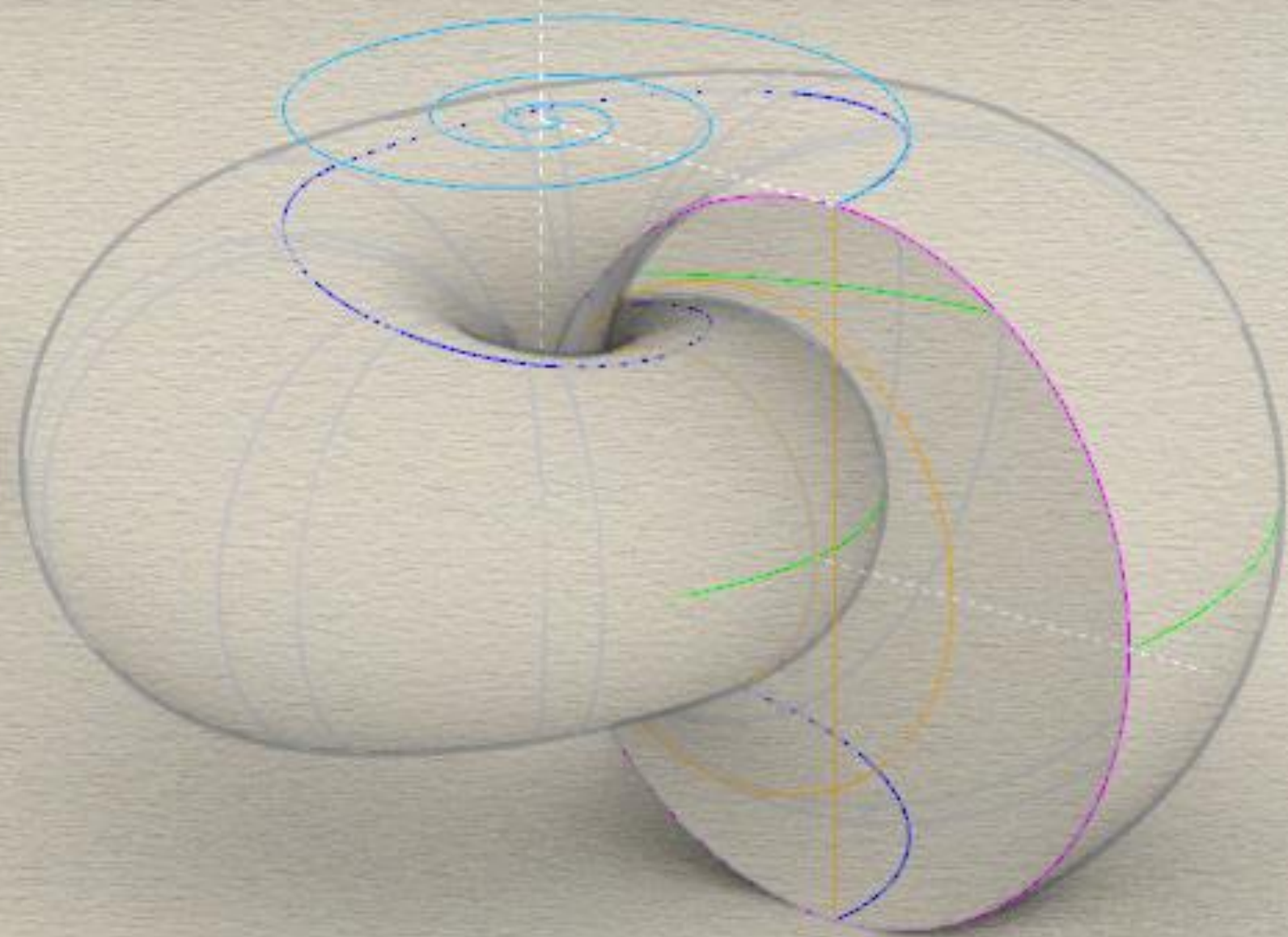
Ex:2.3 - Nautilus
