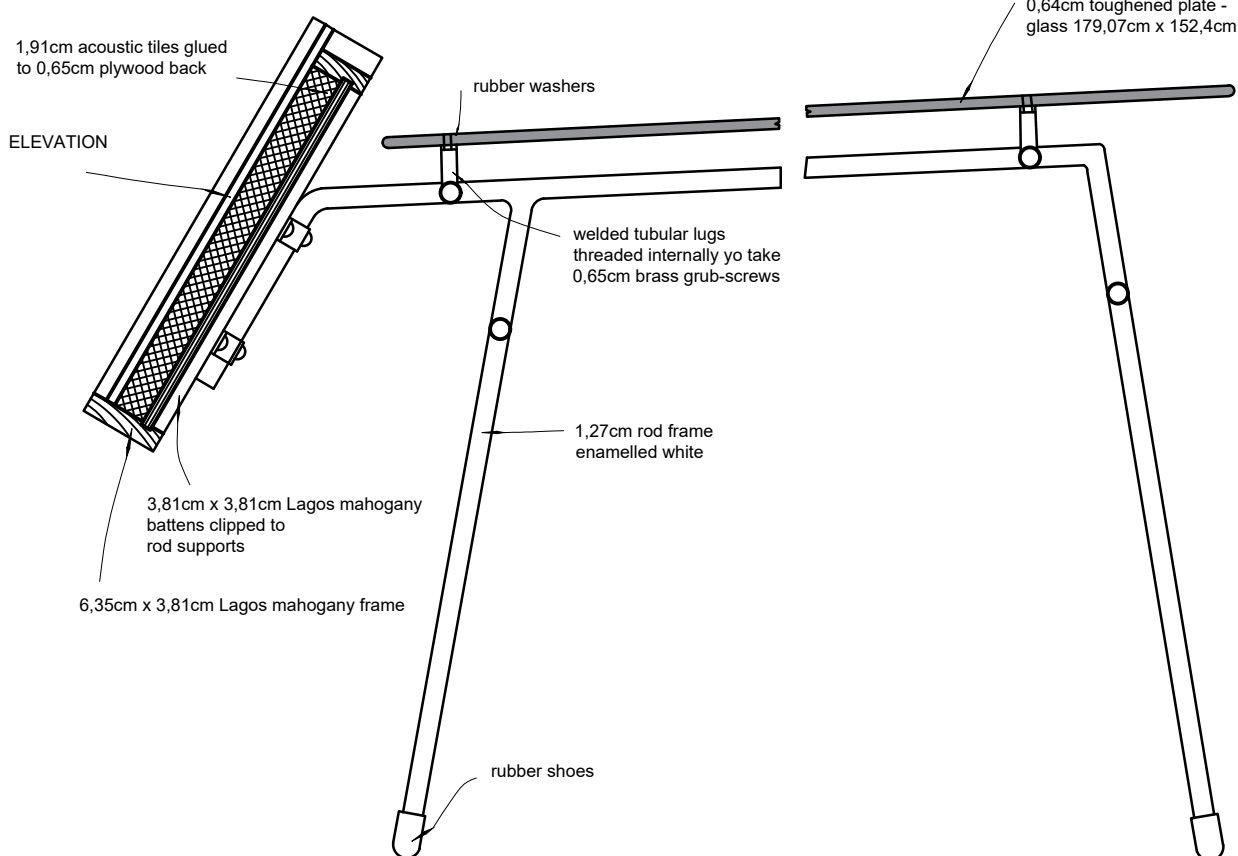
SECTION THROUGH DISPLAY UNIT.
